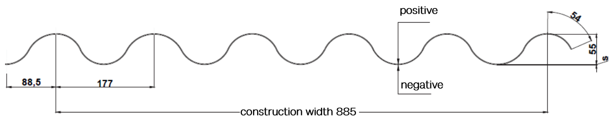
roof/wall installation
