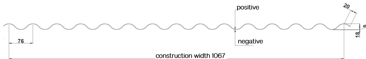
wall installation
